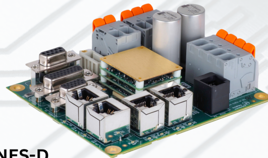
NES-D Development Board
